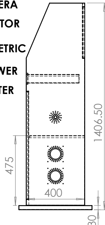
RH SIDE VIEW
